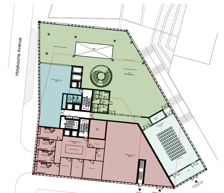
Library first floor layout
