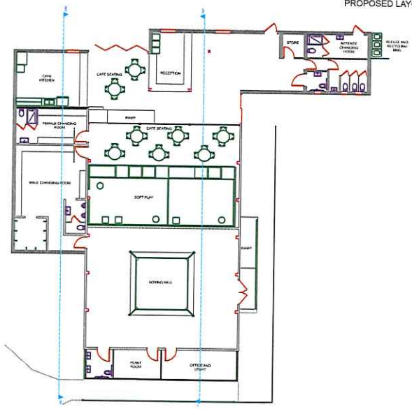
01 FLOOR PLAN 1:100
